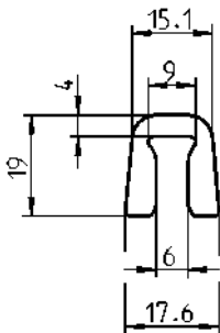
Clip-on profile EPDM 60 ± 5 Shore A, of fire protection compound, black
