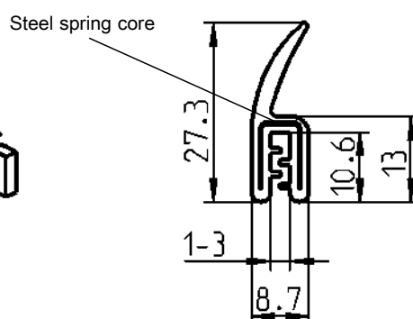
Sealing profile and clamping profile EPDM 60 ± 5 Shore A, black
