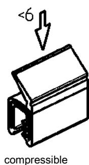
Sealing profile EPDM, clamping profile EPDM 60 ± 5 Shore A, black
