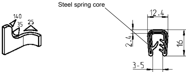
Edge protection made of fire protection compound EPDM 60 ± 5 Shore A, black ① 1010-S19-FR01
