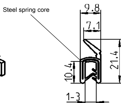
Sealing profile EPDM, clamping profile EPDM 60 ± 5 Shore A, black
