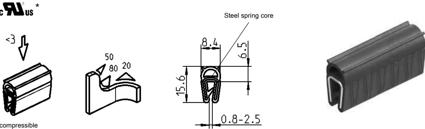
Sealing profile sponge rubber and clamping profile material of your choice
