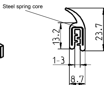
Sealing profile and clamping profile EPDM 60 ± 5 Shore A, black
