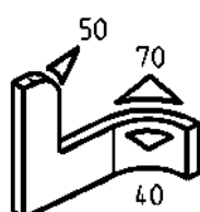
Sealing profile EPDM, clamping profile EPDM 60 ± 5 Shore A, black
