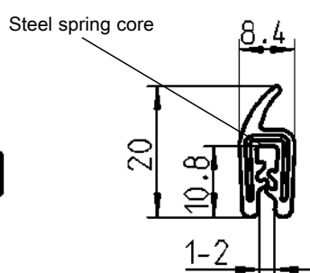
Sealing profile and clamping profile EPDM 60 ± 5 Shore A, black
