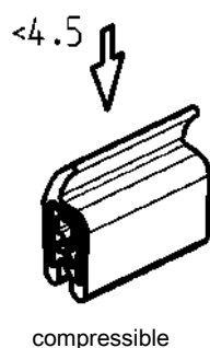
Sealing profile and clamping profile EPDM 60 ± 5 Shore A, black
